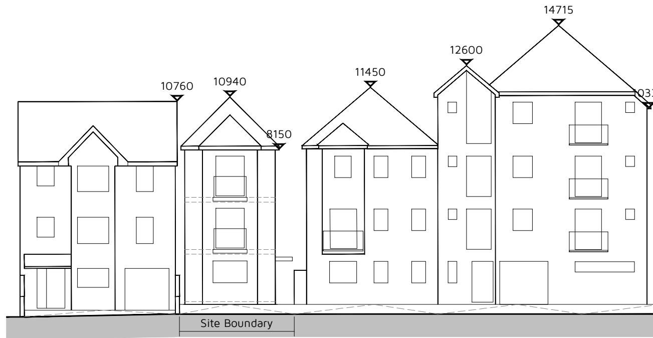
Illustrative Proposed Street Scene Elevation 1:200 @ A3
